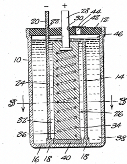
U.S. Pat. No. 2,322,210: Battery
