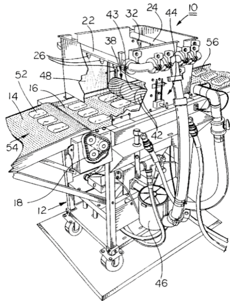
(b) U.S. Pat. No. 5,762,968: Method and Apparatus for Producing Imitation Grill Marks on Food Without Using Heat
