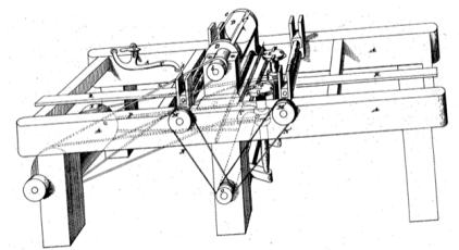
U.S. Pat. No. U.S. Pat. No. Reissue 71 : Improvement in Machines for Planing, Tonguing, Grooving, and Dressing Boards, &c.
