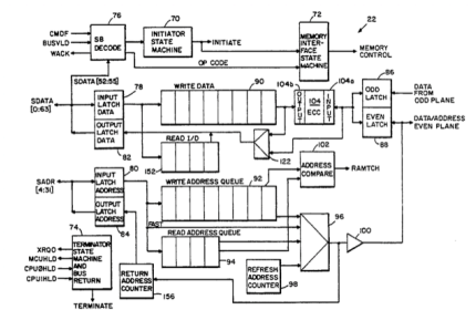
U.S. Pat. No 5,379,379 : Memory Control Unit with Selective Execution of Queued Read and Write Requests:
