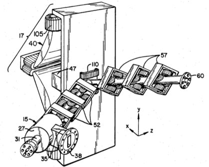
U.S. Pat. No 4,641,103: Microwave Electron Gun
