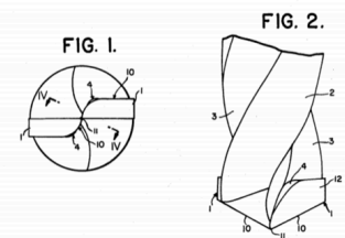
U.S. Pat. No 4,222,690: Drill Having Cutting Edges with the Greatest Curvature at the Central Portion Thereof
